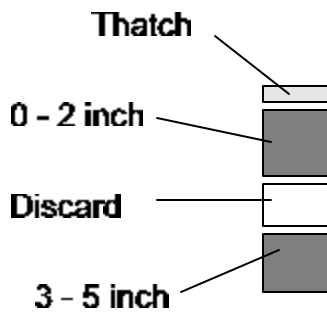
Figure. Illustration of sample core sections used for electrical conductivity evaluation.
